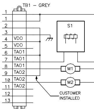
TYPICAL OUTPUT WIRING
