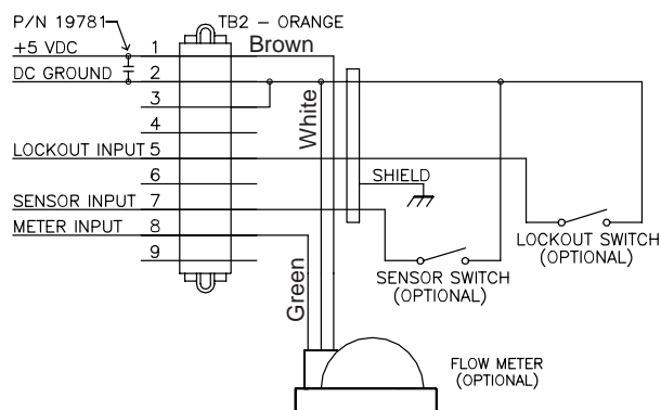
TYPICAL INPUT WIRING
