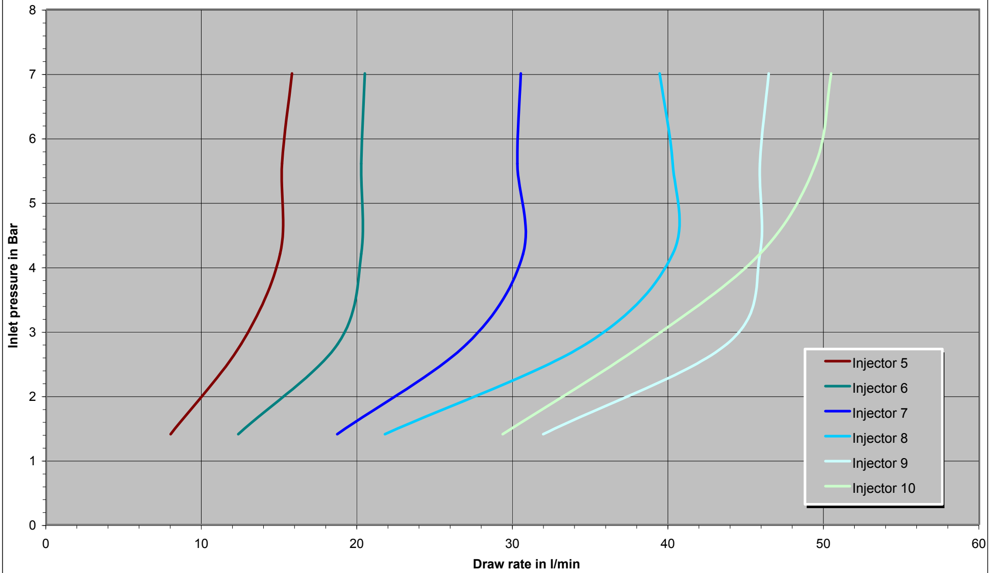
Draw rates for 1800 series injectors
