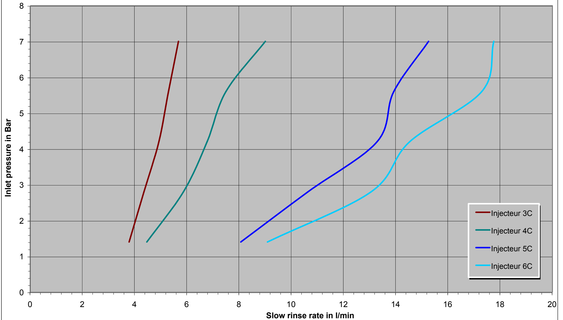
Rinse rates for 1700 series injectors
