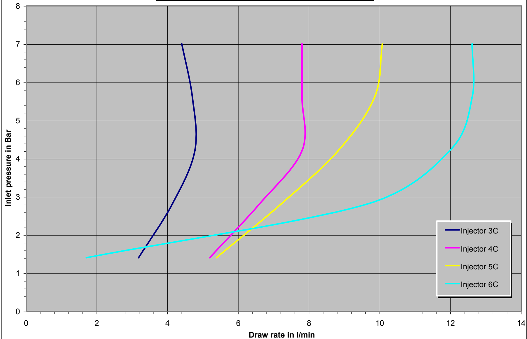
Draw rates for 1700 series injectors
