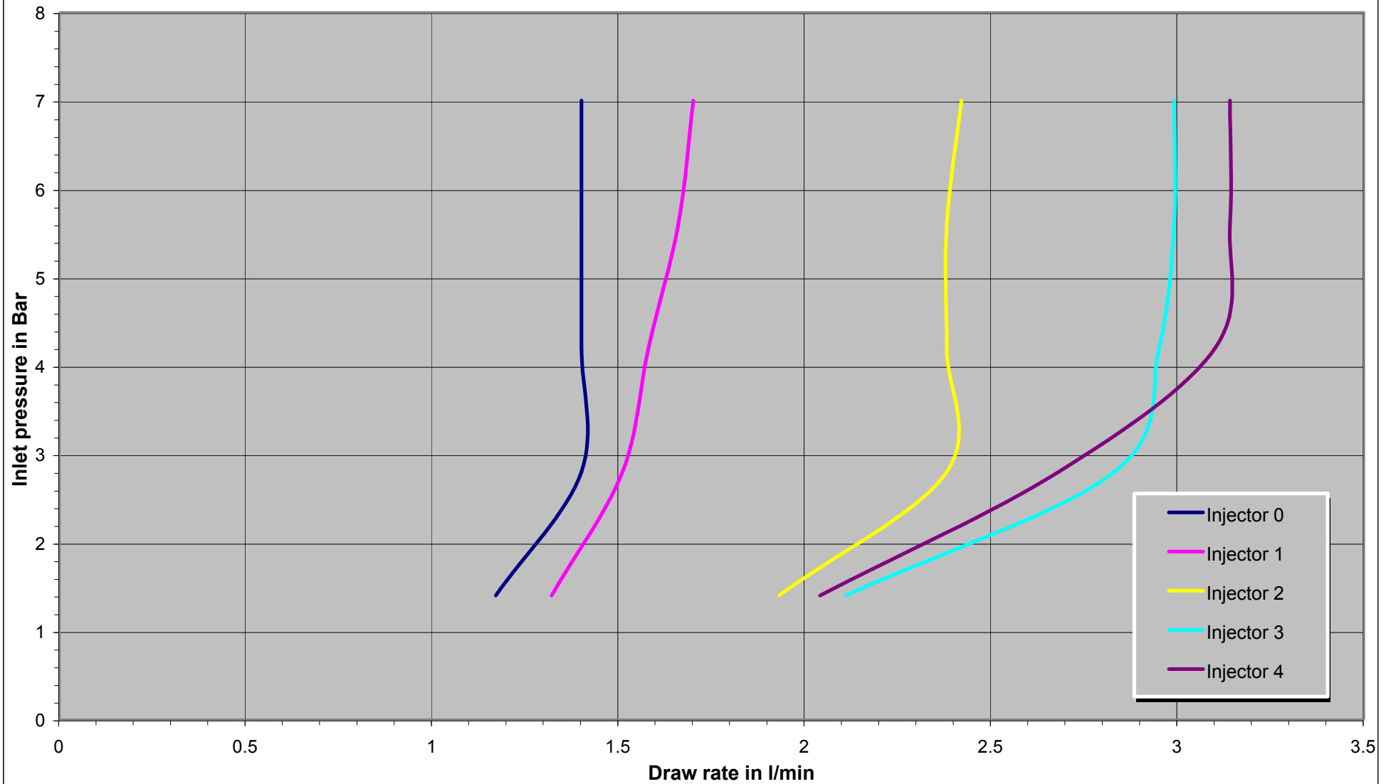
Draw rates for 1600 séries injectors
