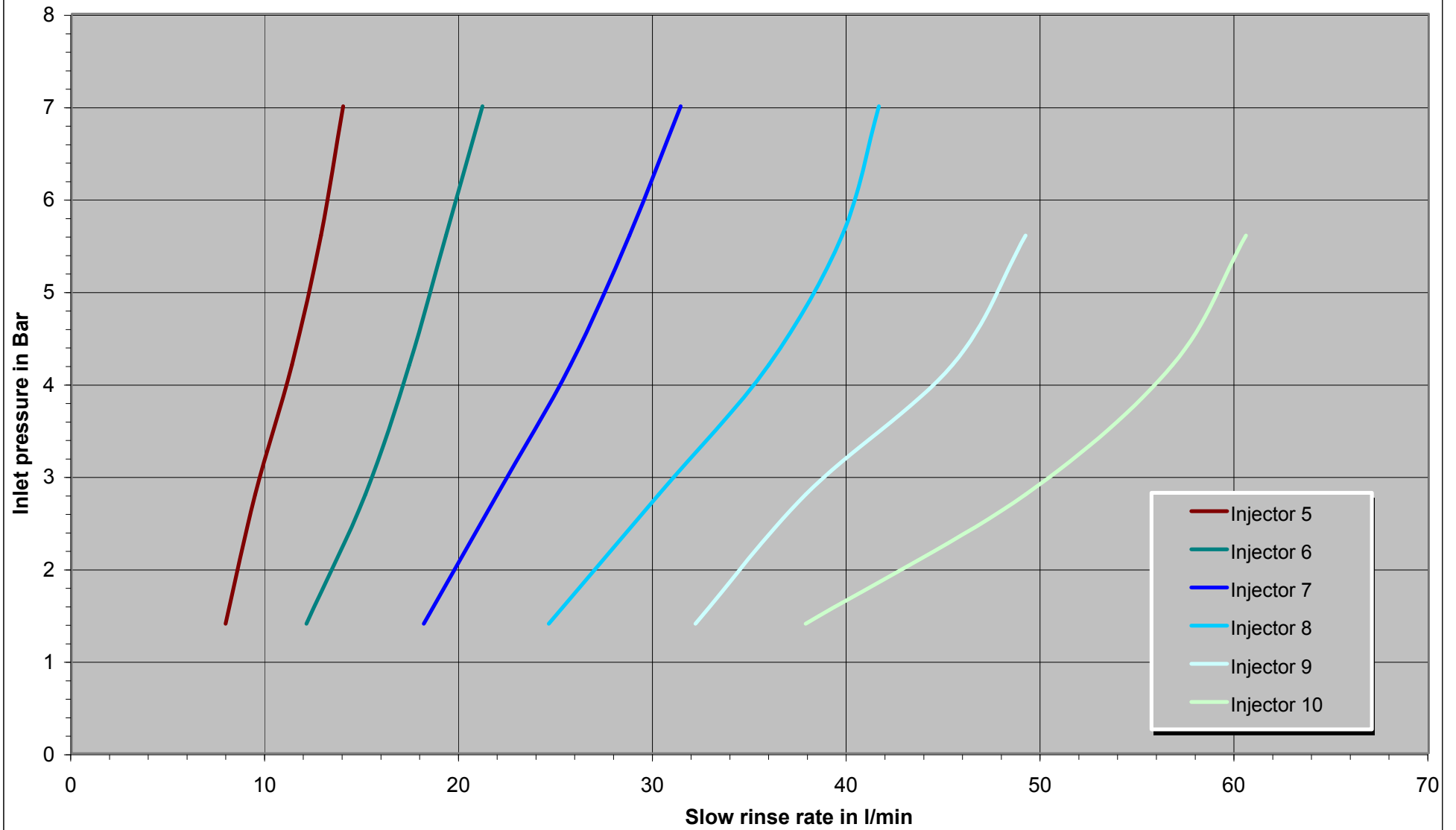
Rinse rates for 1800 series injectors
