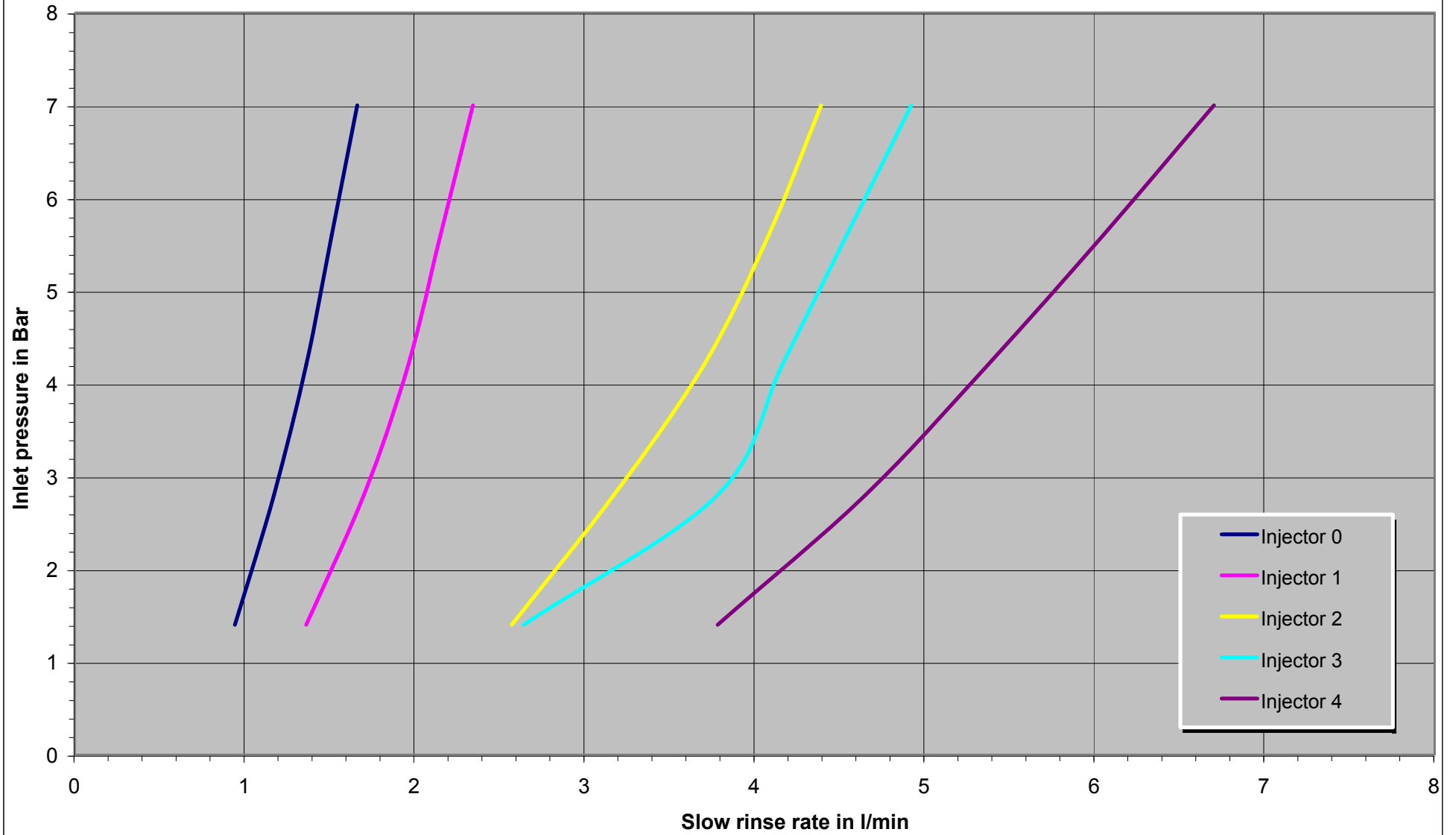
Rinse rates for 1600 series injectors
